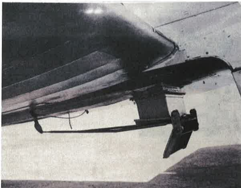
Figure 9 Release valve, also identified as “special tank outlet” on Tanker #1, Floyd Nolte’s Boeing Stearman Model 75, location unknown, 1955; George Nolte Collection
